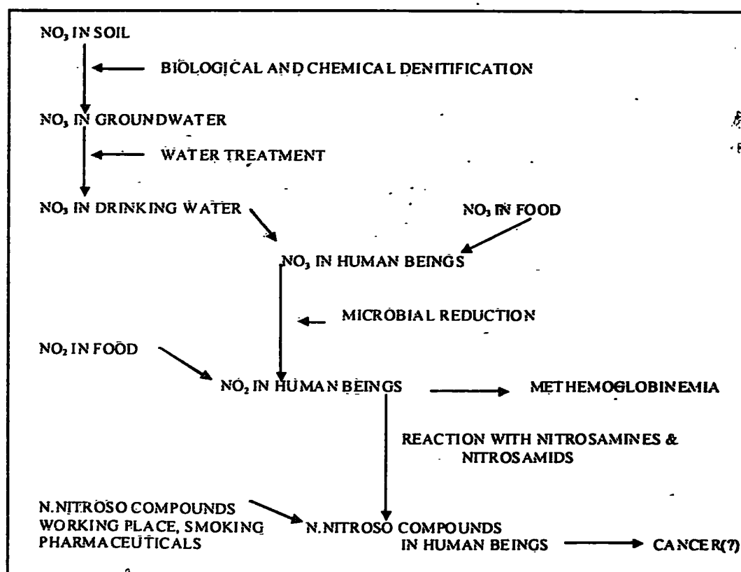
Figure 1: Nitrate pathways and metabolism (Paul and Clark, 1989)
