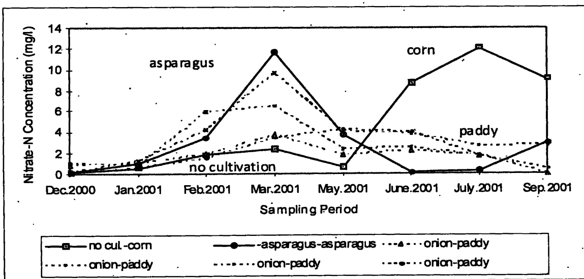
Figure 8: Variation of nitrate concentration in shallow well samples with crop type (Shiroishi Plain, Japan)
