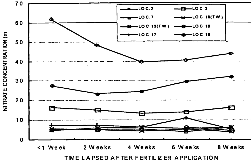
Figure 4: Variation of nitrate in groundwater with time after application of fertilizer(Udunuwara area, Kandy)
