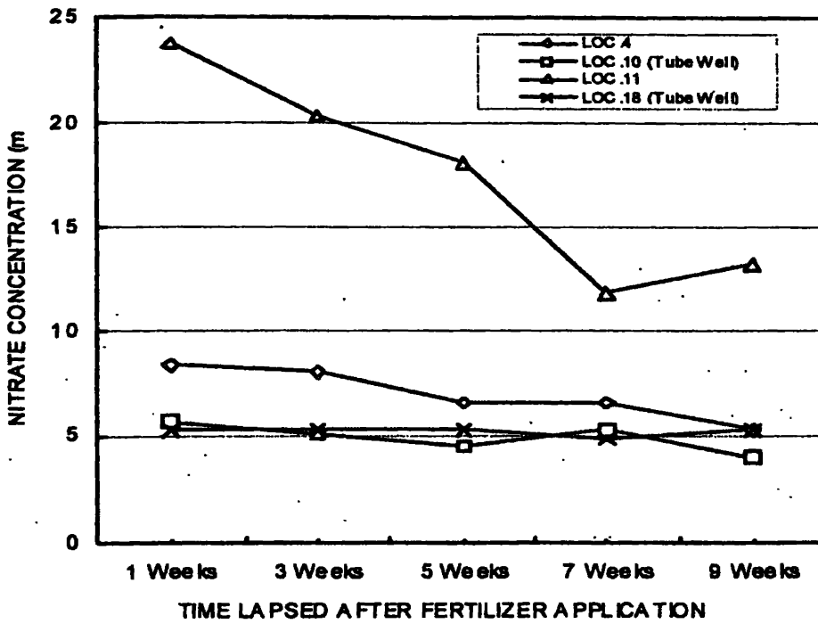
Figure 6: Difference between the variation of Nitrate in tube wells and dug wells (Udunuwara area, Sri Lanka)
