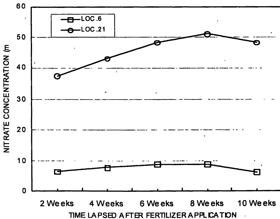
Figure 5: Tendency of decreasing nitrate levels after few weeks, as a result of groundwater flow (Udunuwara area, Sri Lanka)
