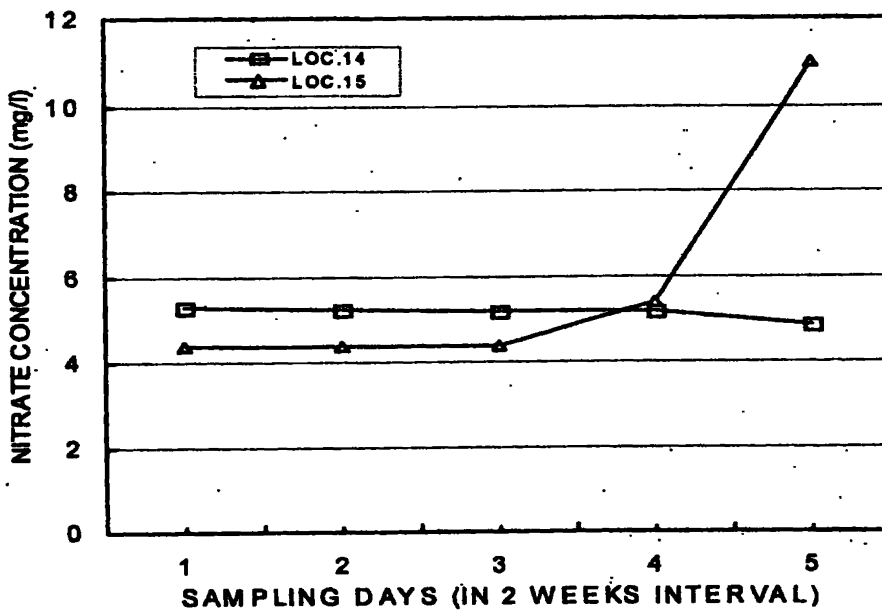
Figure 7: Behavior of Nitrate concentration Vs. time (Udunuwara area, Sri Lanka)
